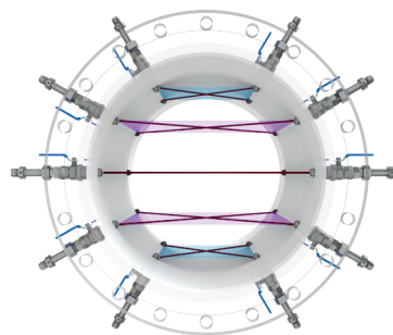
Wetted sensors arranged in five parallel planes
