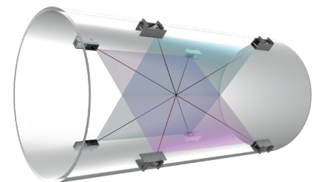
Clamp-On sensors arranged in two 45° planes
